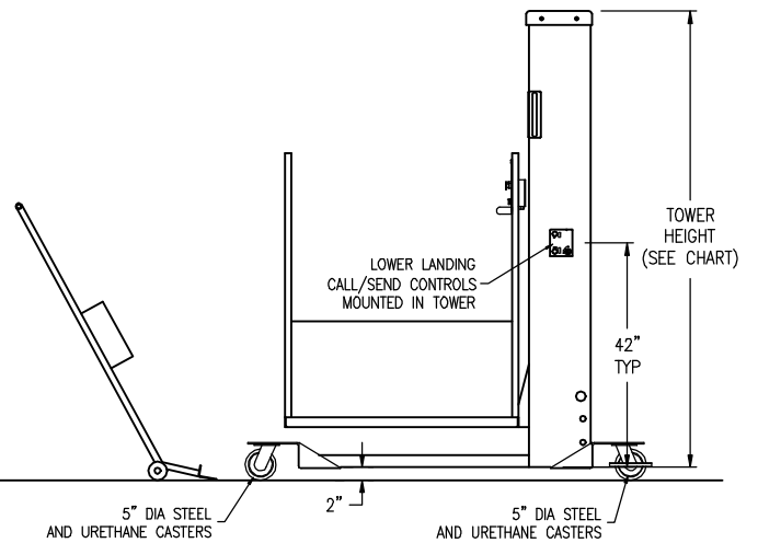
LOWER LANDING SIDE ELEVATION
