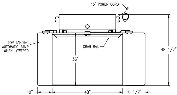
RUNNING CLEARANCES
