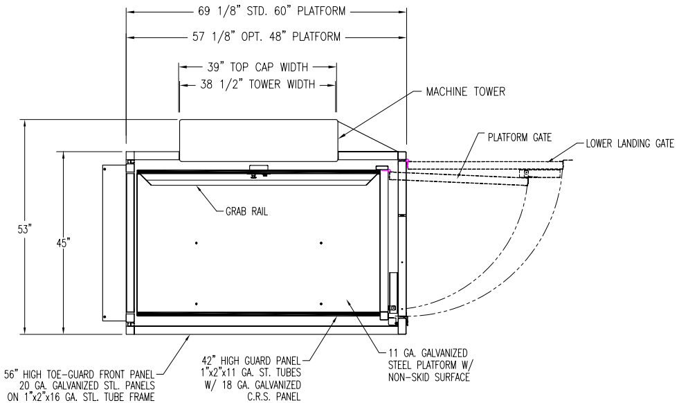
PLAN VIEW
